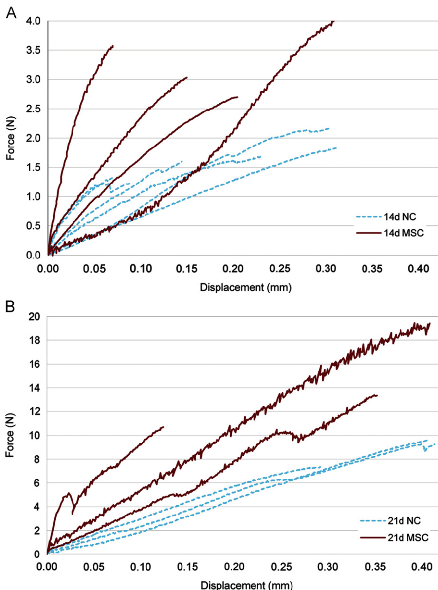
Fig. 3. Biomechanical testing force vs. displacement plot for (A) 14 day post-fracture calluses without MSC transplantation and 14 day post-fracture with MSC transplantation, (B) 21 day post-fracture calluses without MSC transplantation and 21 day post-fracture with MSC transplantation.
